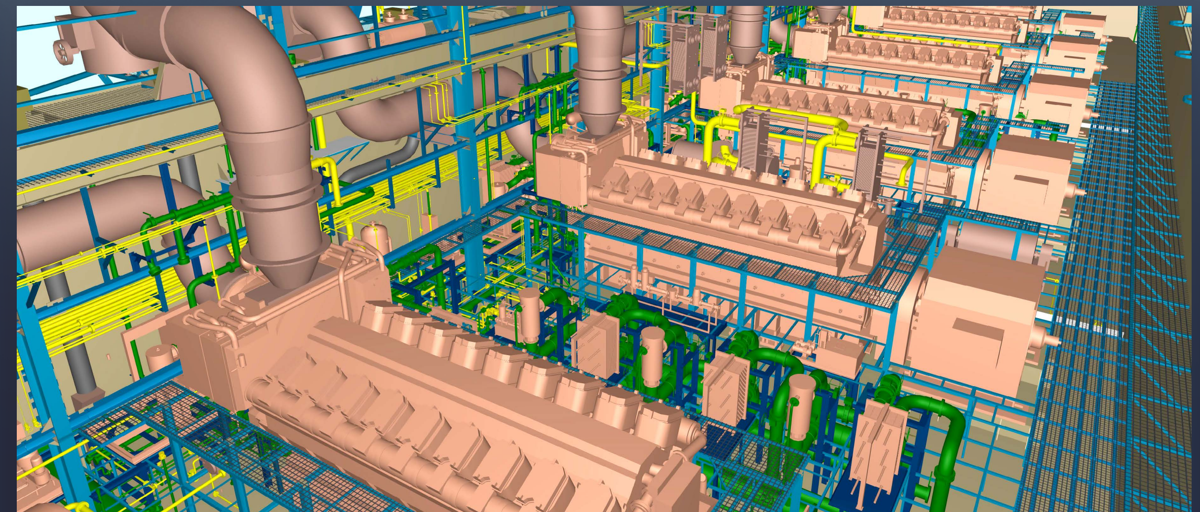
KPS-6 POWERSHIP
