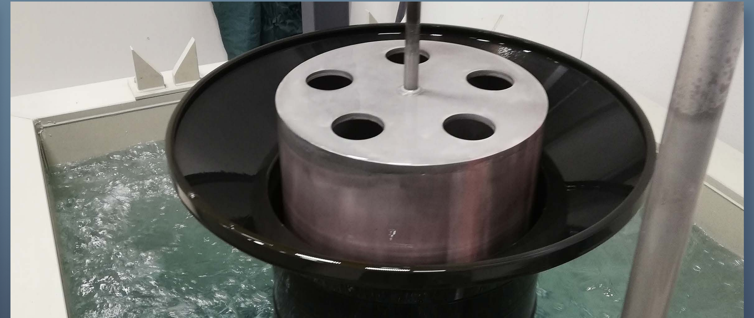
MACRO ETCH
