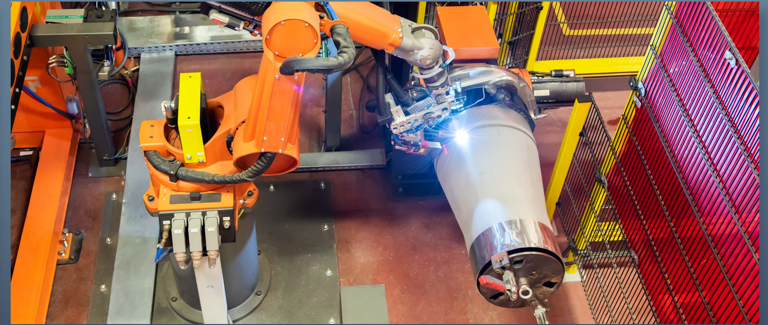
COLD METAL TRANSFER (CMT) ADDITIVE WELDING
