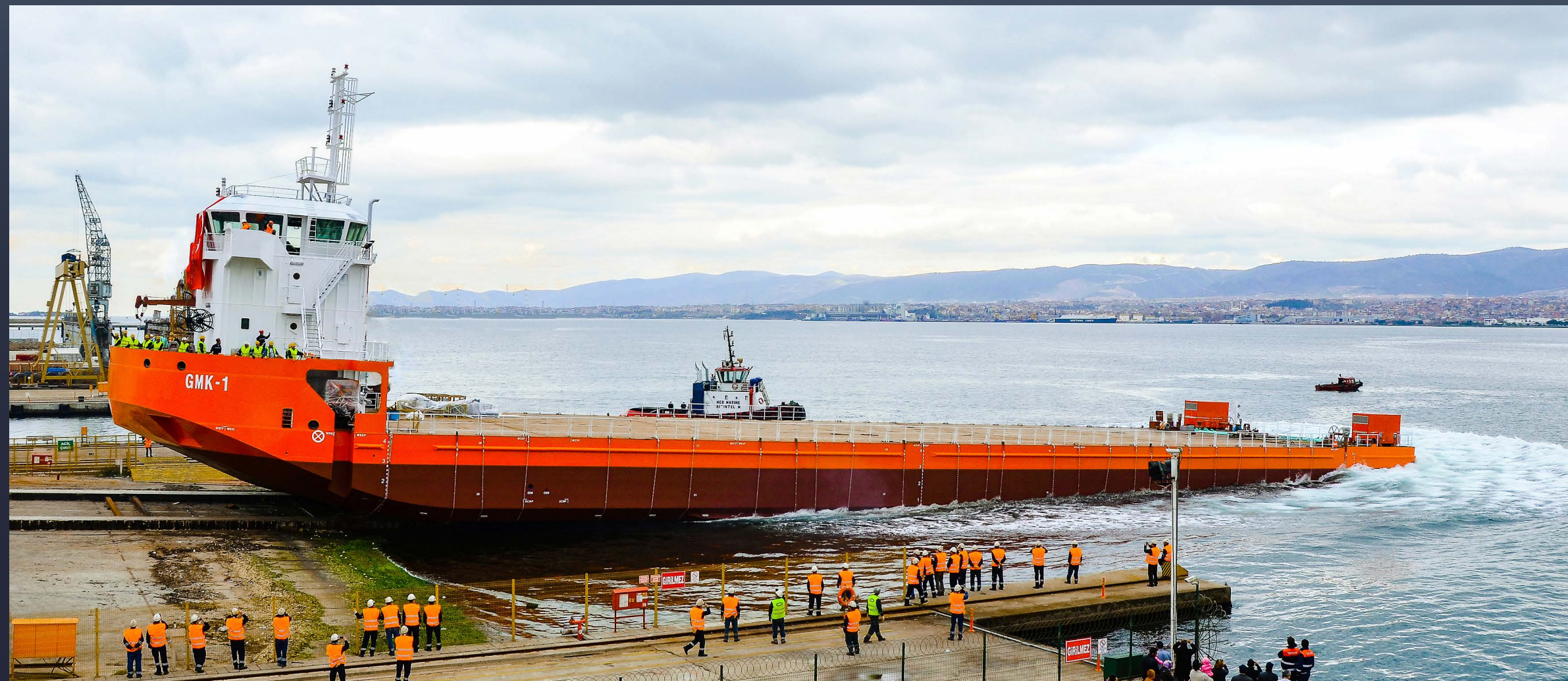
GMK-1 DYNAMIC POSITIONING SERVICE VESSEL
